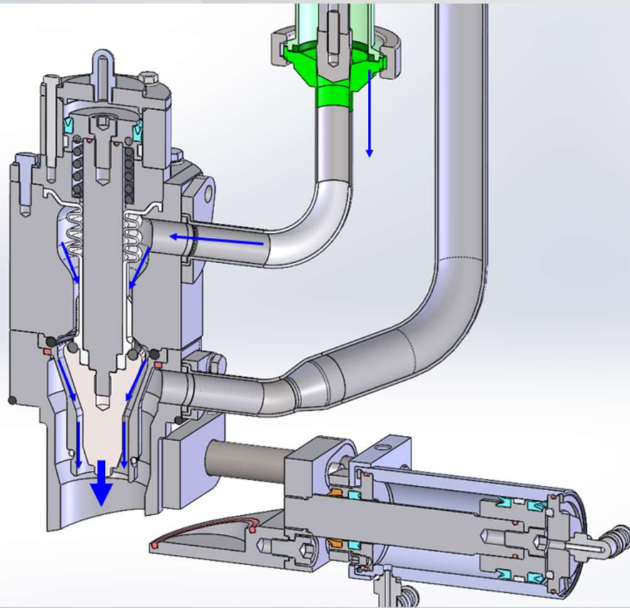
Filling cycle
