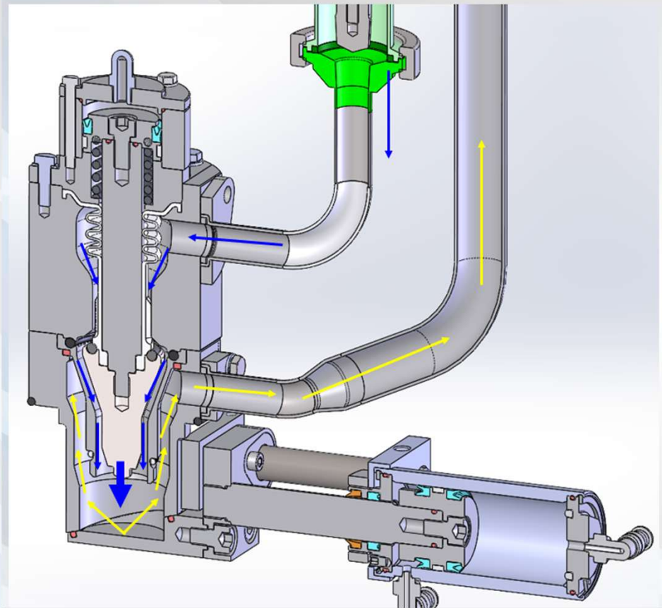
CIP cycle
